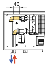
PR40 – extension piece 40 mm, 2×elbow 90° All other models FRT, FRK, except for the ones stated with PR50
