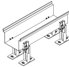
Heater with mounted legs
