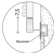
Wireless connection with Standard Edge Cap
