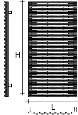
RADIATOR - GVR connection diagram in the standard OR1 configuration with low connectors
