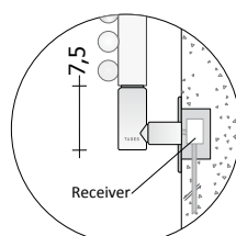
Wireless connection with DESIGN edge cap painted in the same colour (supplied with an extra charge)
