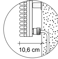
RADIATOR - GVR connection diagram in the standard OR1 configuration with low connectors
